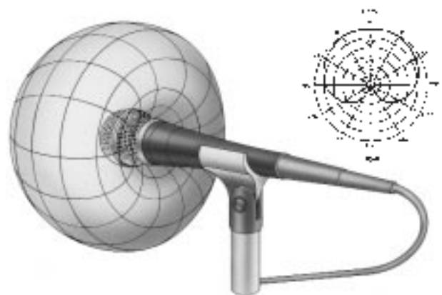
Cardioid (Unidirectional) Microphone
