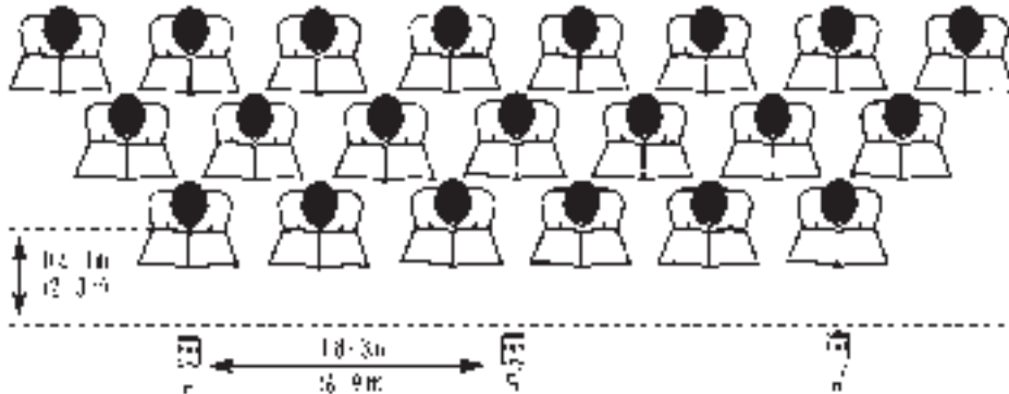
Choir Microphone Positions - Top View
