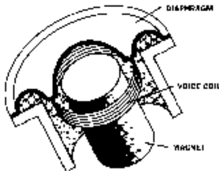
Dynamic Microphone
