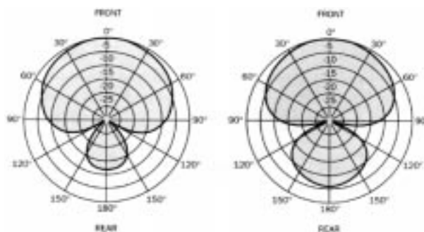
Supercardioid pattern Hypercardioid pattern
