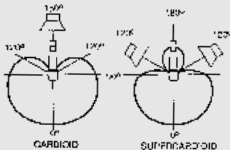
maximum rejection: cardioid and supercardioid
